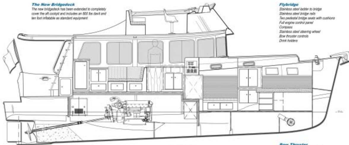
DECK PROFILE
